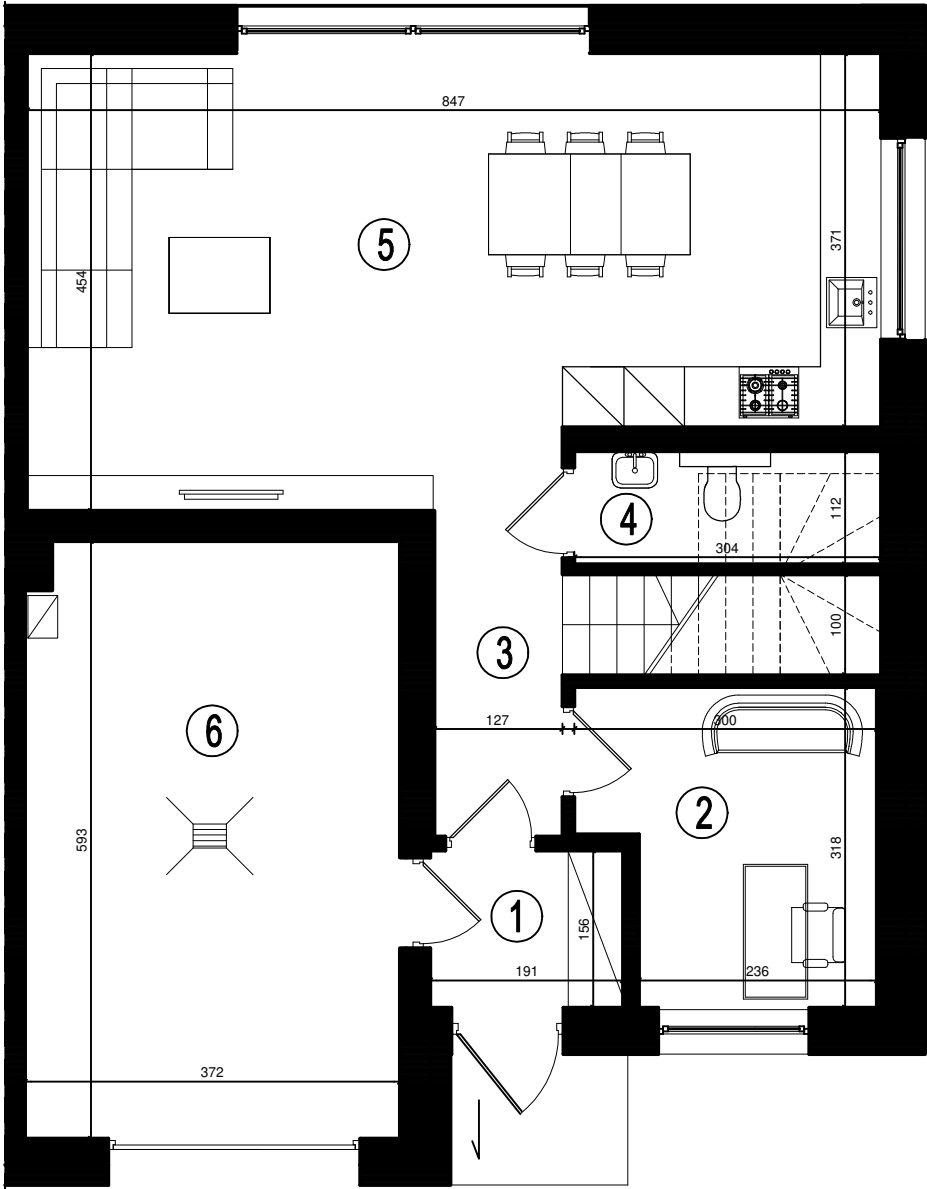
PARTER
